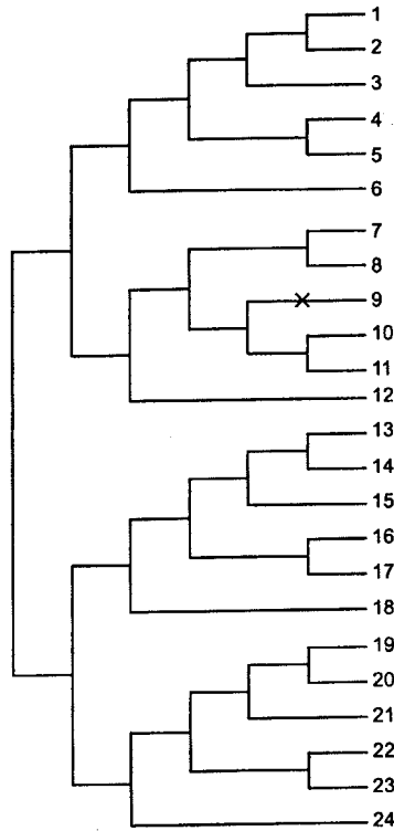
(B) Weighted parsimony
