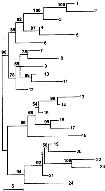
FIGURE 7.11. (A) Standard parsimony tree for simulated sequence data as inferred by the stepwise-addition with “closest” option in PAUP* (no branch swapping). Bootstrap values are shown in boldface (100 replications). (B) Weighted parsimony for the same data set ( w = 5 was used). The branching pattern of sequence 9 is incorrect (see Figure 6.8A).
