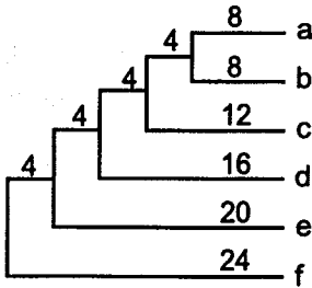
(A) Model tree
