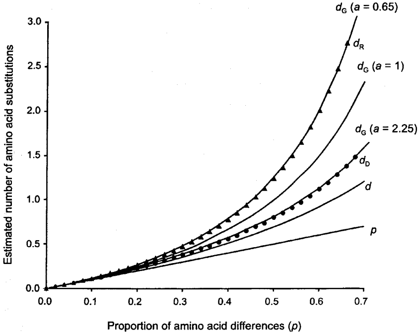
FIGURE 2.4. Relationships of various distance measures with the proportion of amino acid differences ( p ). Dots indicate the Dayhoff distance ( d_D ), whereas triangles stand for the Grishin distance ( d_R ).
