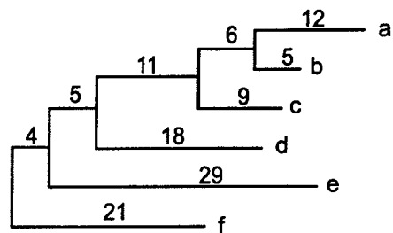
(B) Realized tree
