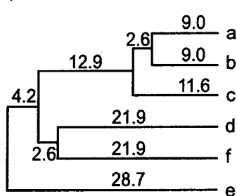
FIGURE 5.5. (A) Model tree, (B) realized tree, and (C–F) reconstructed trees. The neighbor-joining, maximum likelihood, and UPGMA trees were constructed with the Jukes-Cantor model. The branch lengths of the maximum parsimony tree were estimated by the average pathway method.
