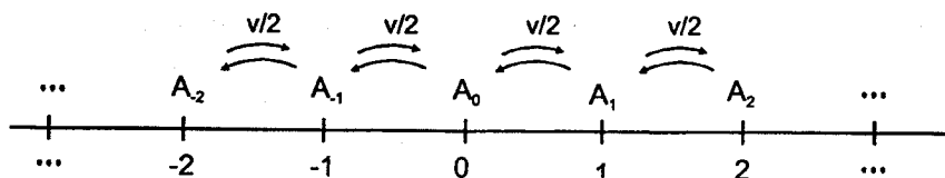
FIGURE 12.2. Stepwise mutation model.
