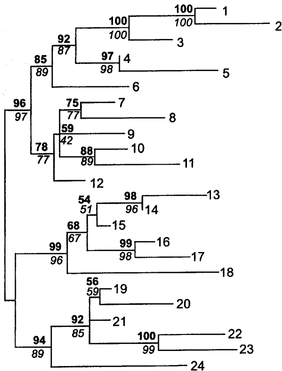
FIGURE 8.4. Maximum likelihood tree for simulated sequence data as inferred by the NJ + NNI search with the Kimura model in PAUP*. Bootstrap values (100 replications) are shown in boldface for the Kimura model and in italics for the Jukes-Cantor model.
