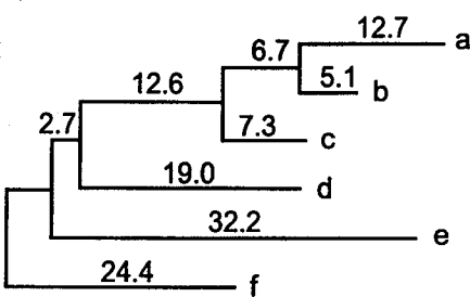
(E) Maximum likelihood tree
