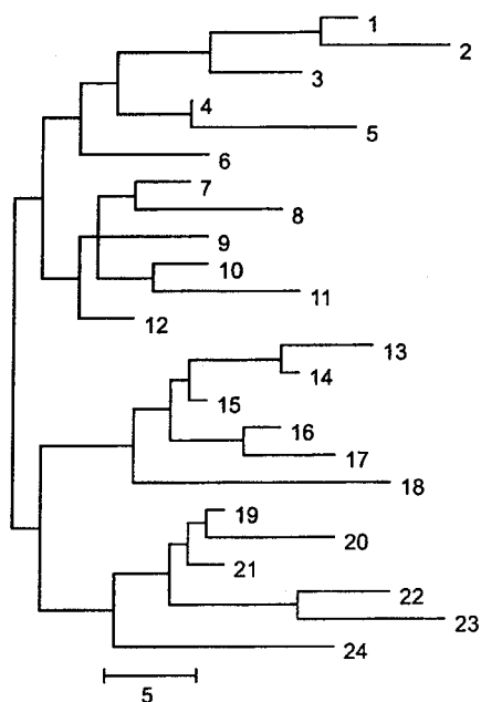
(B) Realized tree
