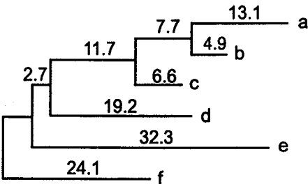
(C) Neighbor-joining tree
