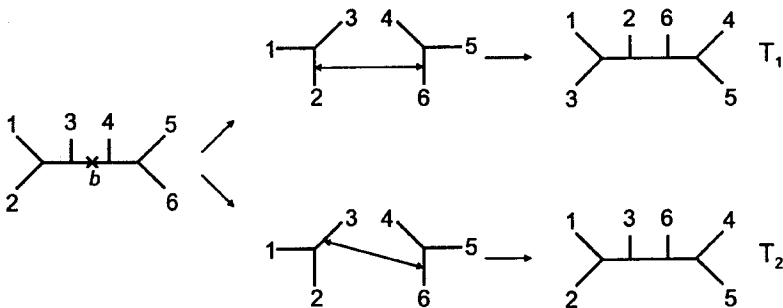
FIGURE 7.6. Three different methods of branch swapping for finding MP trees.
