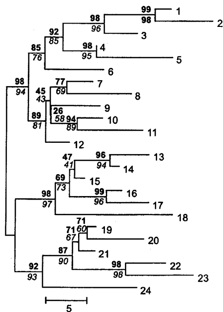
(C) NJ tree with Jukes-Cantor distance
