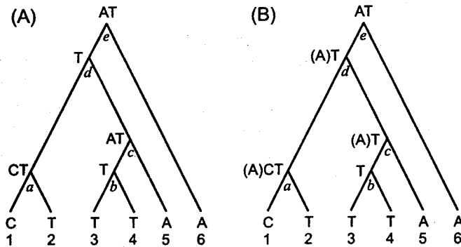
FIGURE 7.1. Nucleotides in six extant sequences and the possible nucleotides in five ancestral sequences.
